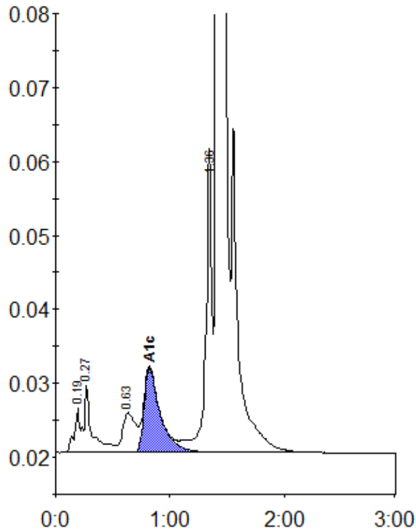
Peak table - ID: 10717829
