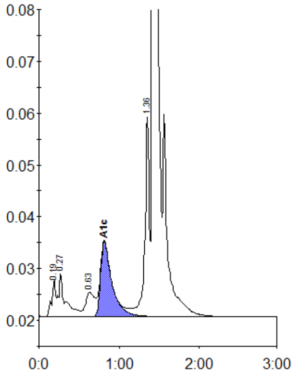
Peak table - ID: 10767614
