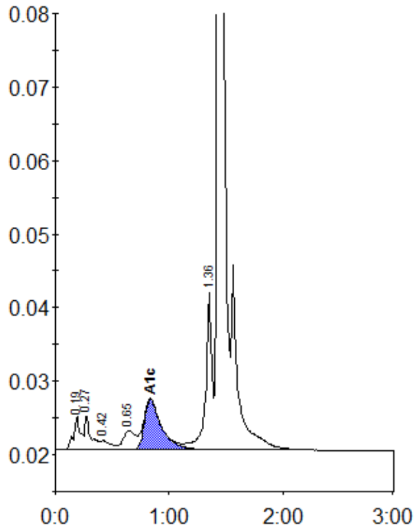
Peak table - ID: 10752981
