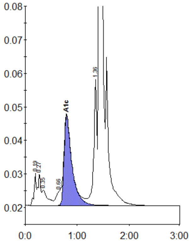
Peak table - ID: 10716099
