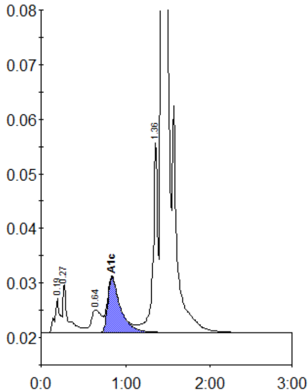
Peak table - ID: 10713768
