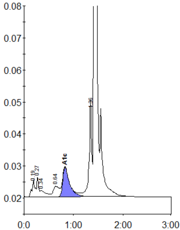
Peak table - ID: 10752991
