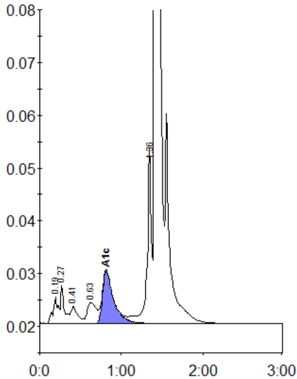
Peak table - ID: 10702641
