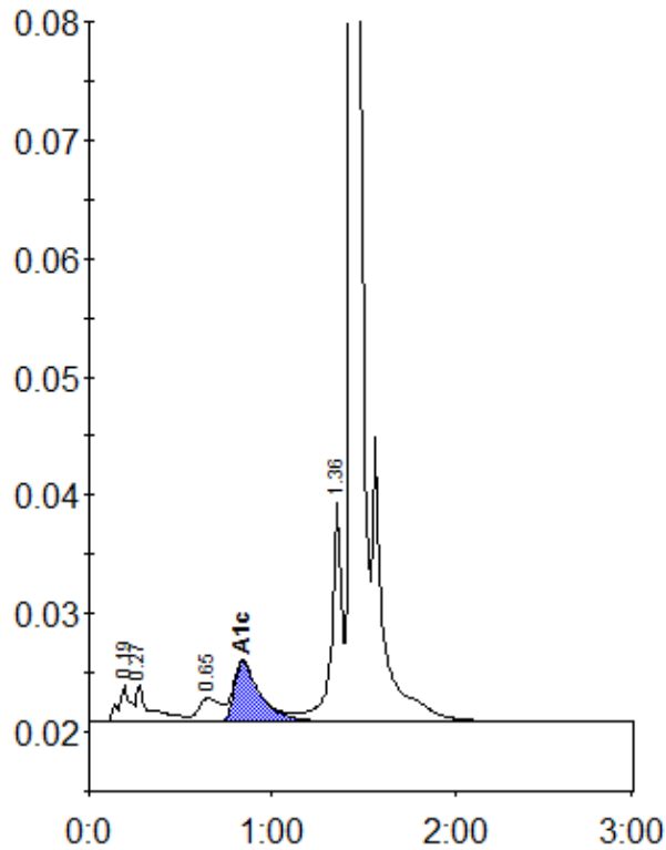
Peak table - ID: 10693994
