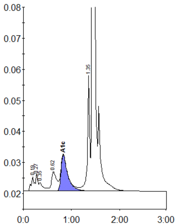
Peak table - ID: 10721143
