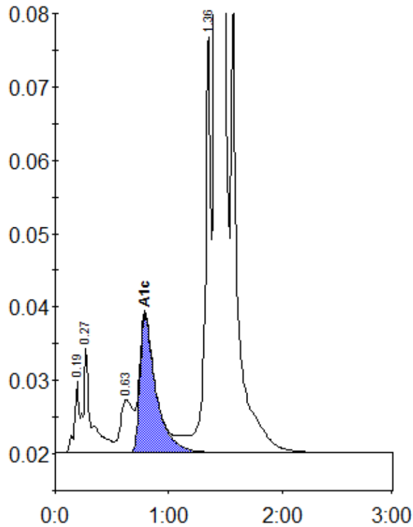
Peak table - ID: 10713208
