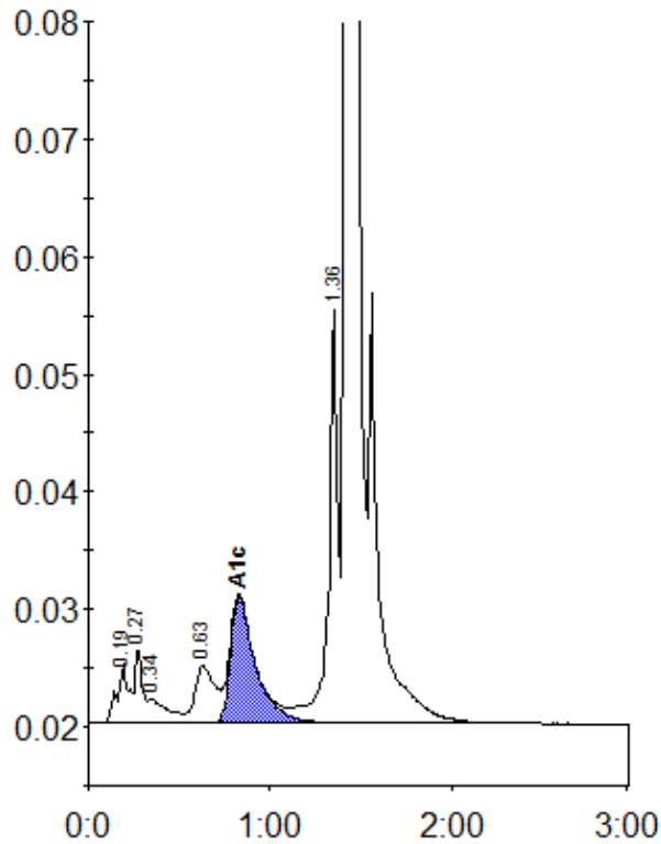
Peak table - ID: 10716243
