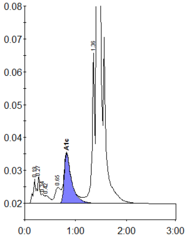
Peak table - ID: 10507470
