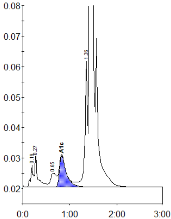
Peak table - ID: 10469320
