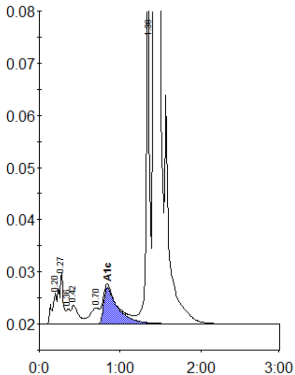
Peak table - ID: 10481338
