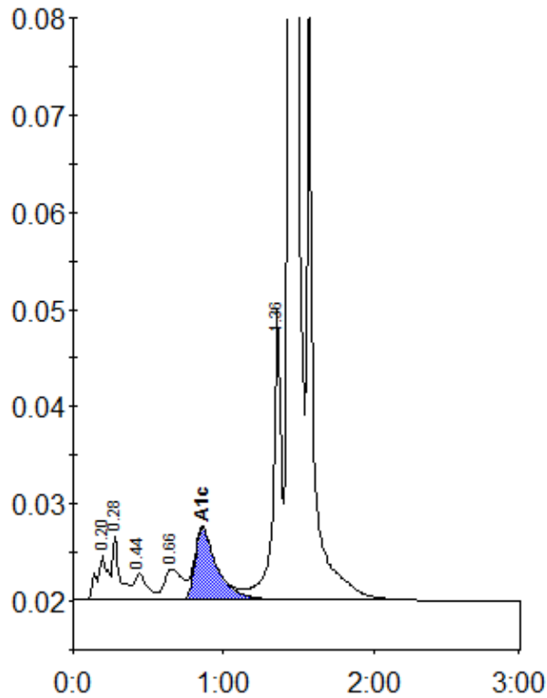
Peak table - ID: 10635617
