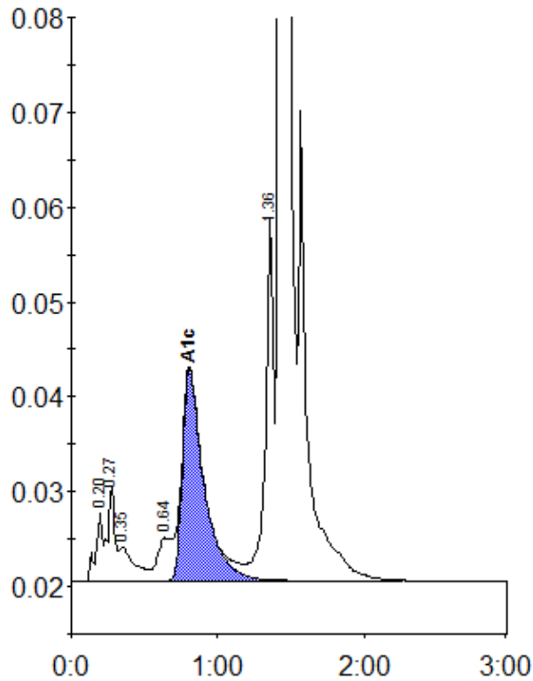
Peak table - ID: 10712804
