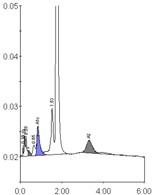
Peak table - ID: 10698120
