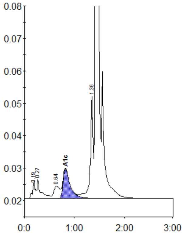
Peak table - ID: 10729511
