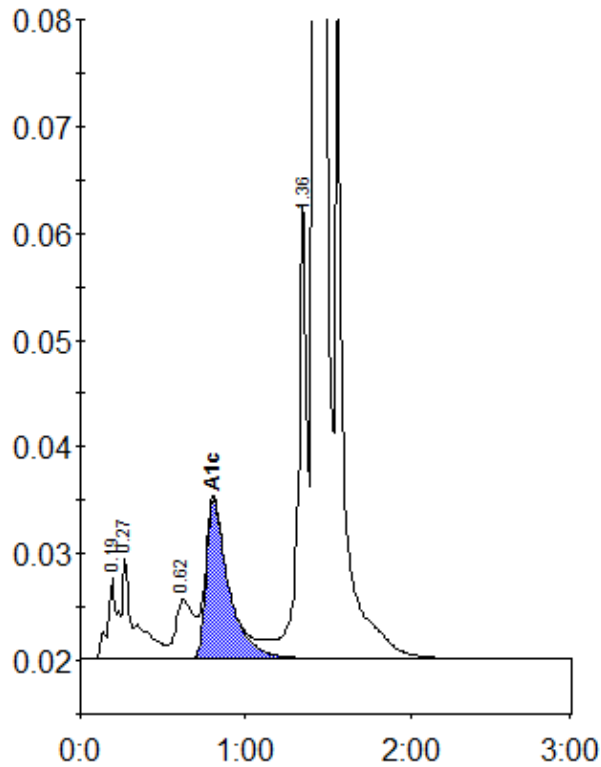
Peak table - ID: 10721785
