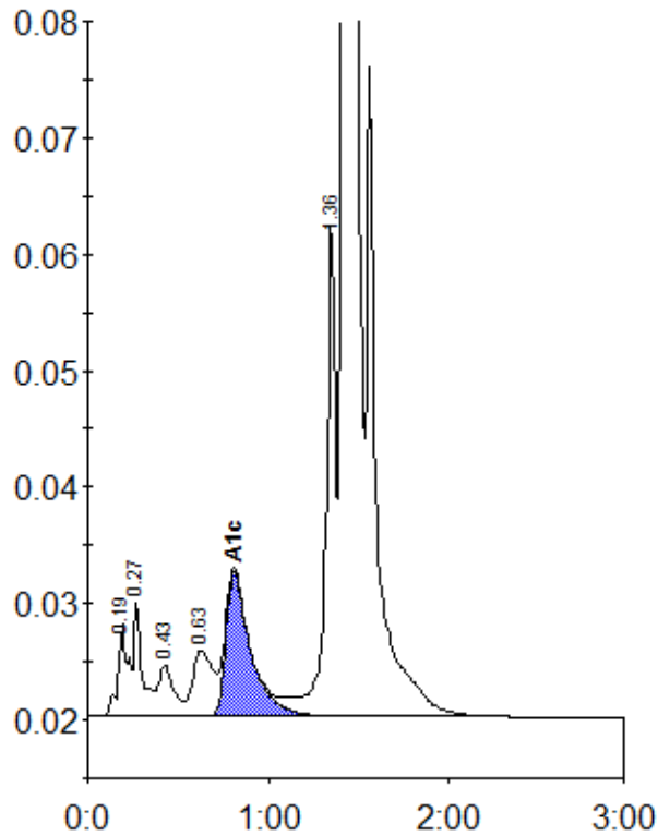
Peak table - ID: 10721790
