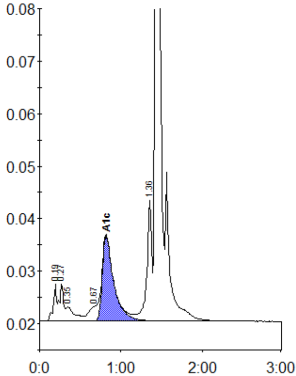
Peak table - ID: 10481149
