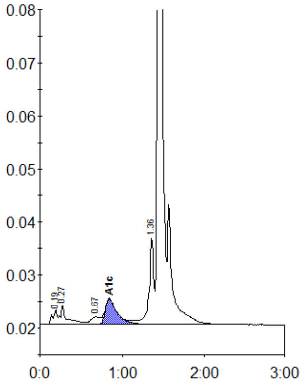
Peak table - ID: 10669456
