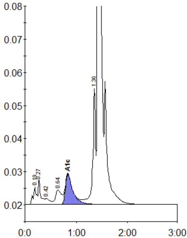
Peak table - ID: 10677668
