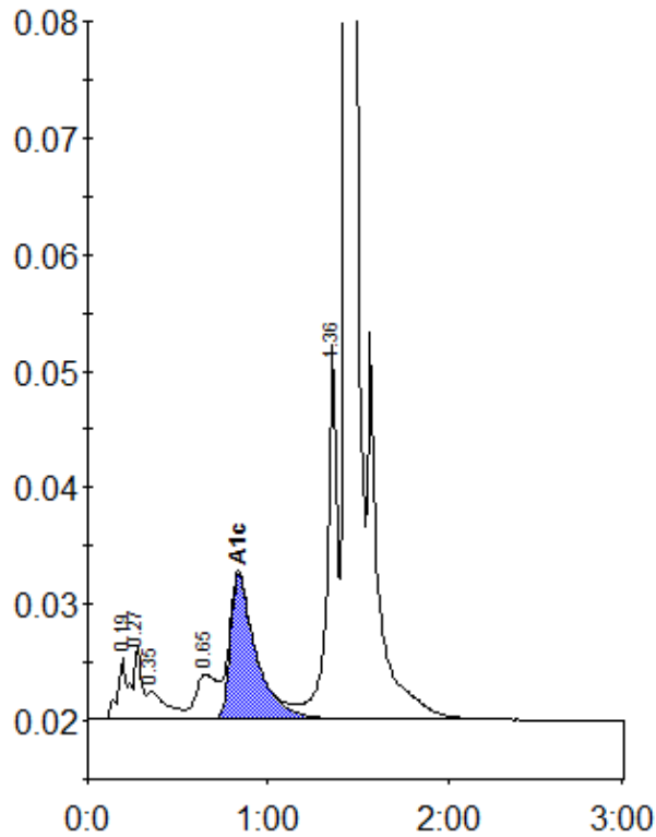
Peak table - ID: 10675857
