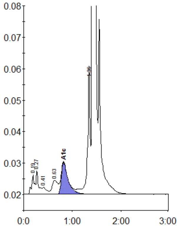
Peak table - ID: 10733883
