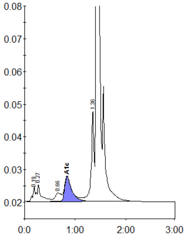
Peak table - ID: 10512860
