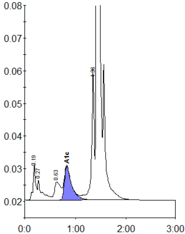
Peak table - ID: 10691120
