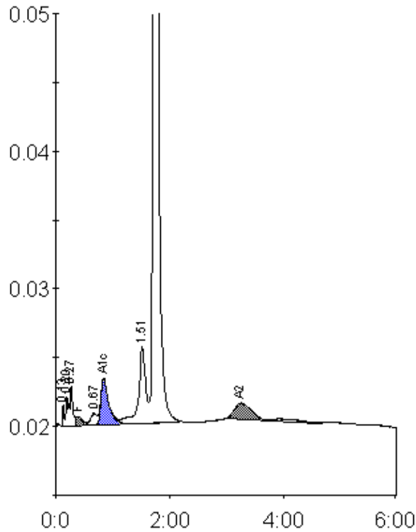
Peak table - ID: 10674620
