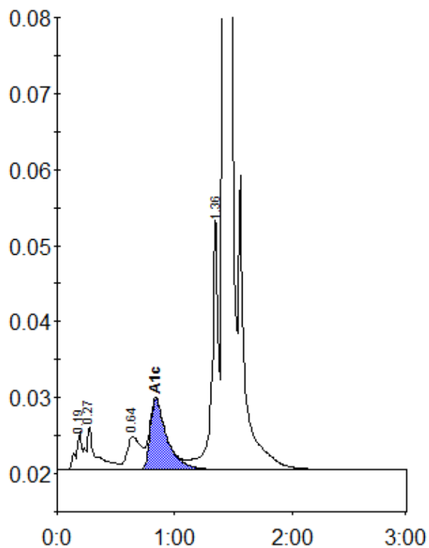
Peak table - ID: 10580593
