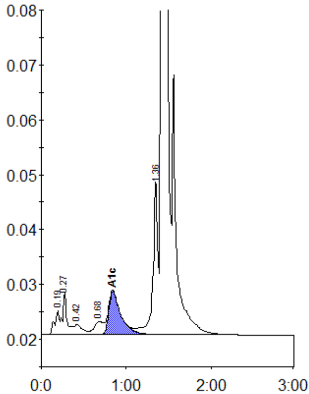
Peak table - ID: 10635290
