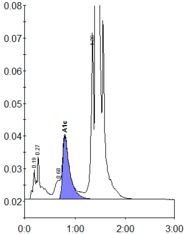
Peak table - ID: 10635520
