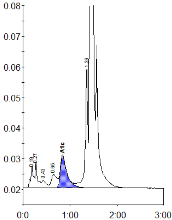
Peak table - ID: 10643047
