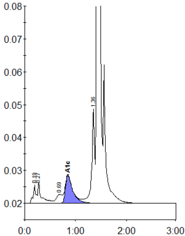
Peak table - ID: 10673643
