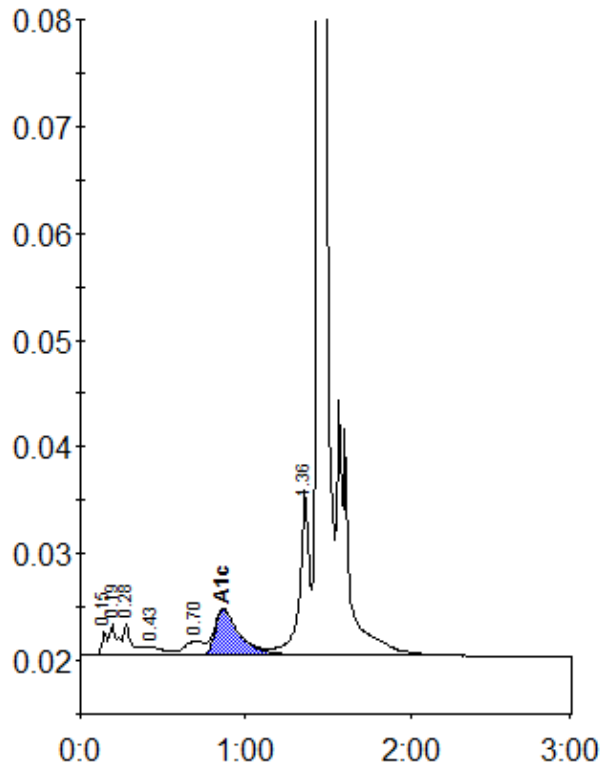
Peak table - ID: 10689700
