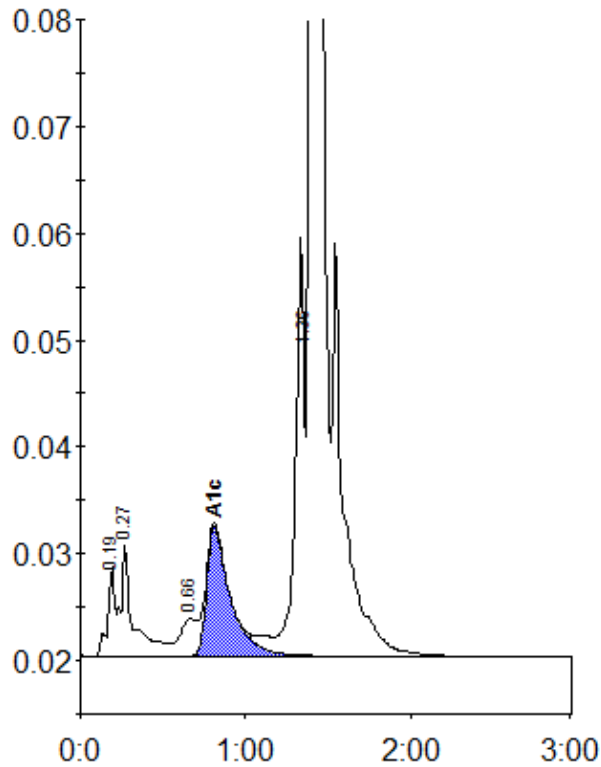
Peak table - ID: 10660723
