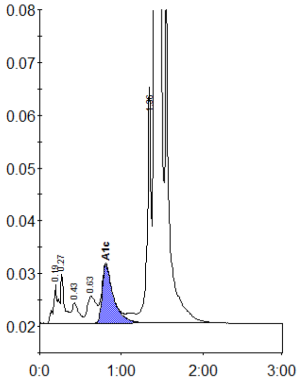
Peak table - ID: 10488845
