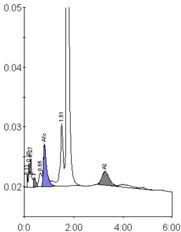
Peak table - ID: 10662267
