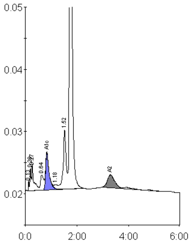
Peak table - ID: 10680926
