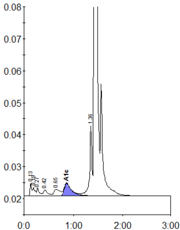
Peak table - ID: 10678049
