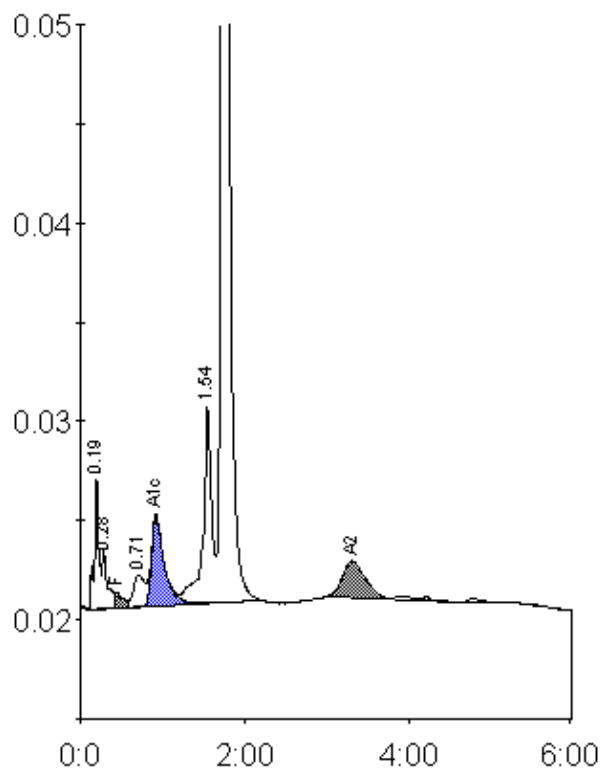
Peak table - ID: 10663174
