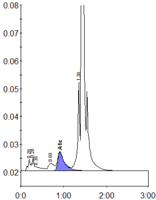
Peak table - ID: 10663366
