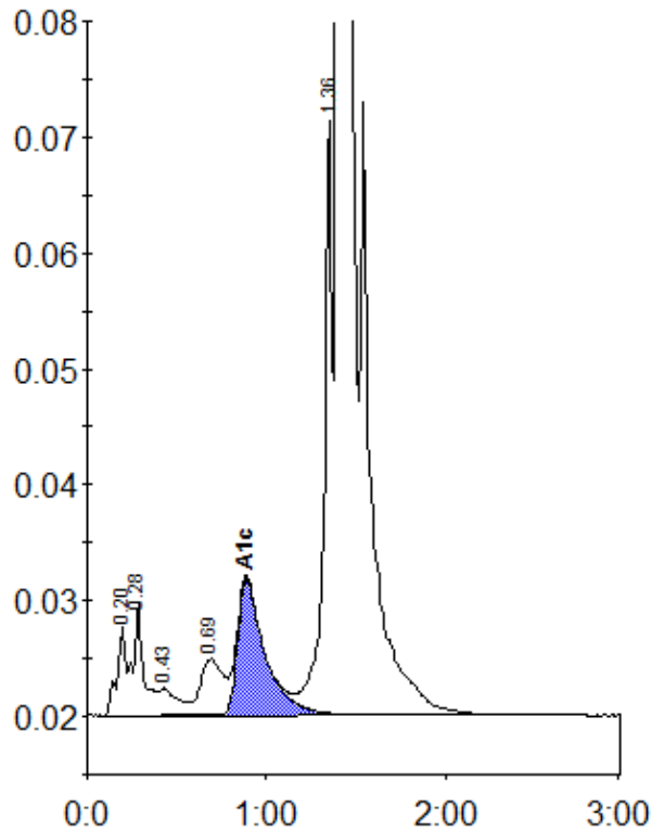
Peak table - ID: 10550377
