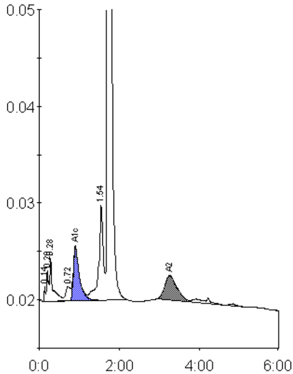
Peak table - ID: 10648445
