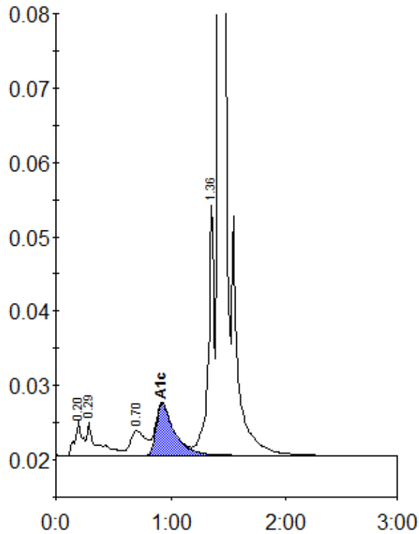
Peak table - ID: 10649332
