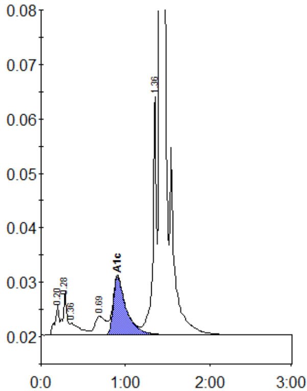
Peak table - ID: 10508972
