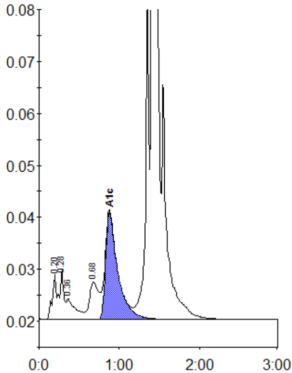
Peak table - ID: 10530708
