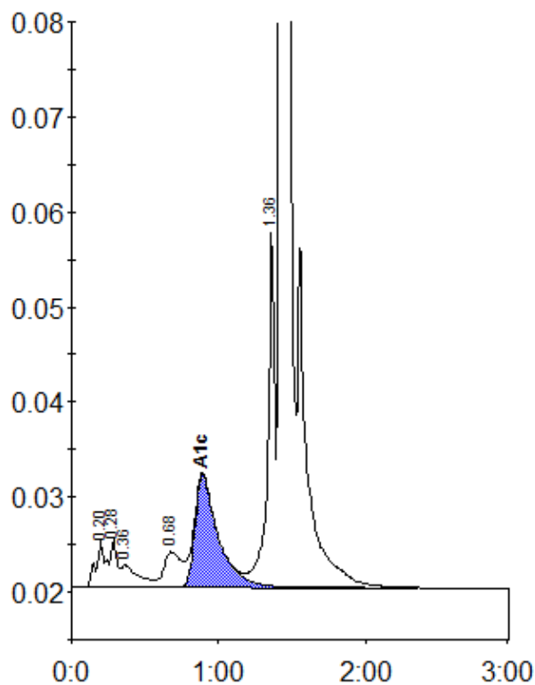
Peak table - ID: 10511001
