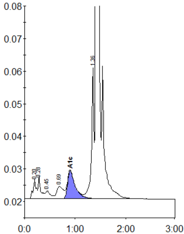
Peak table - ID: 10673225
