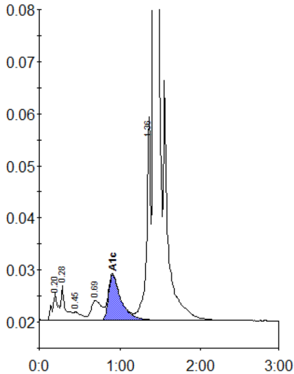
Peak table - ID: 10513403
