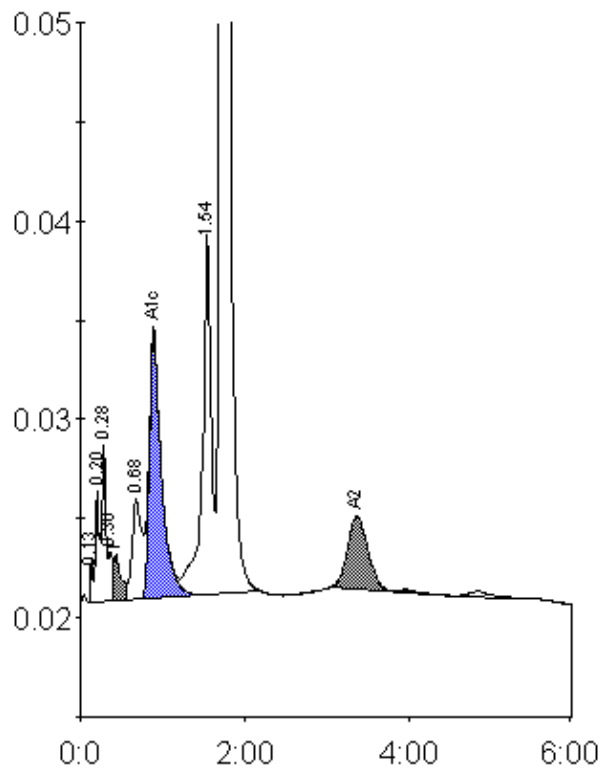
Peak table - ID: 10526812
